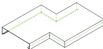
Zed Section
